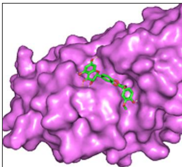
Three-dimensional surface view of \beta -catenin
