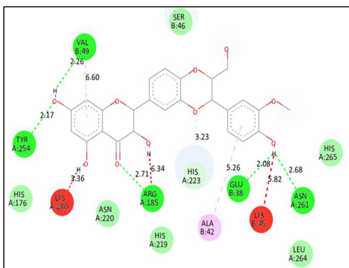
Two-dimensional schematic of the silibinin- \beta -catenin interactions
