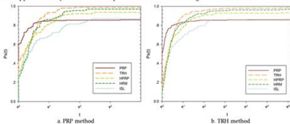
Figure 1. Performance Profile for the Number of Iterations and CPU times.
